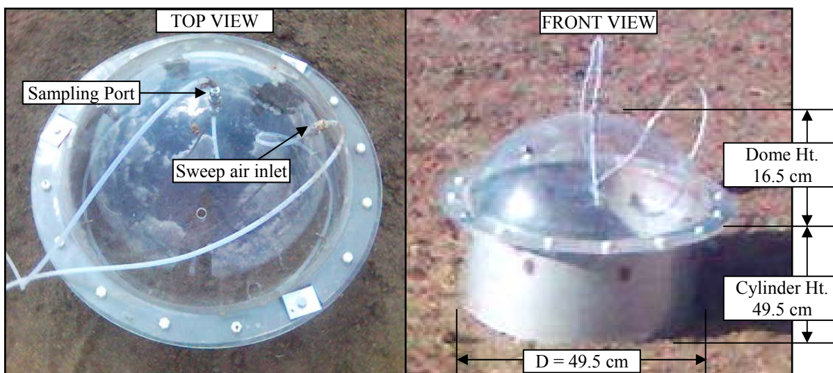
Figure 4. Details of the flux chamber used for air sampling.
