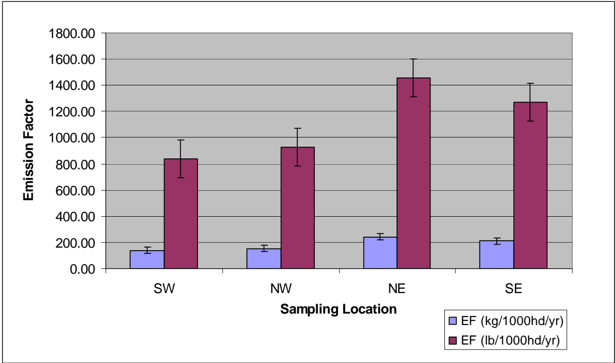
Figure 5. Emission factors of acetic acid from the different locations in the beef cattle openlot.
