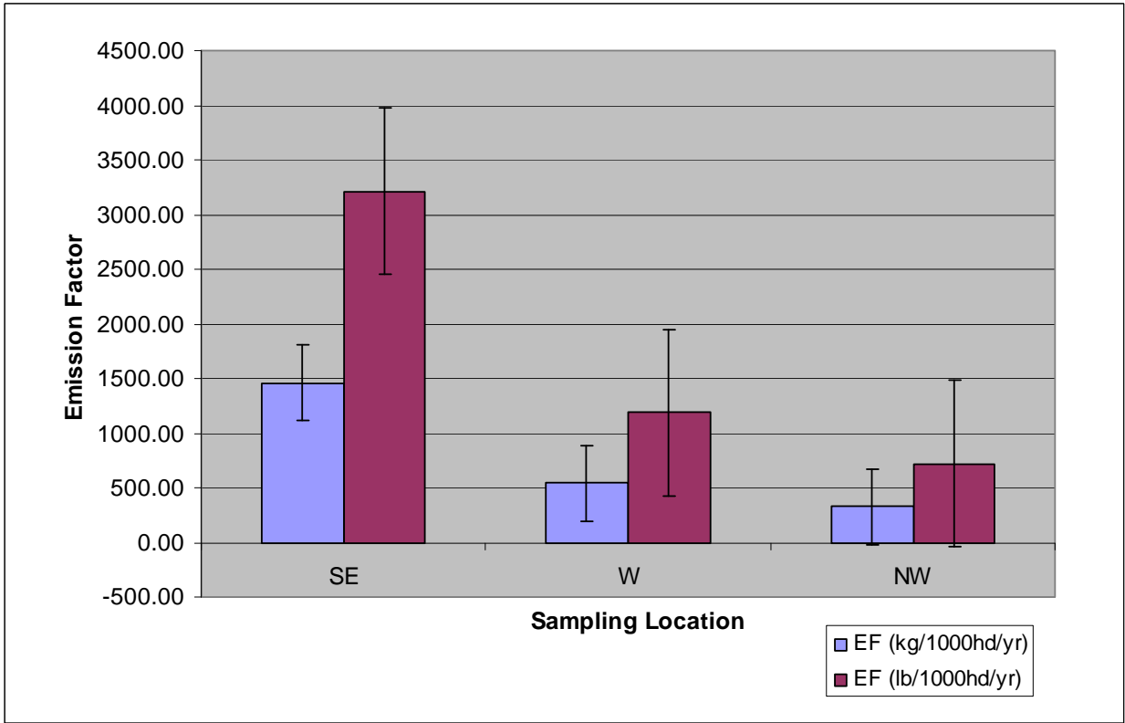
Figure 6. Emission factors of acetic acid from the different locations in the dairy openlot.
