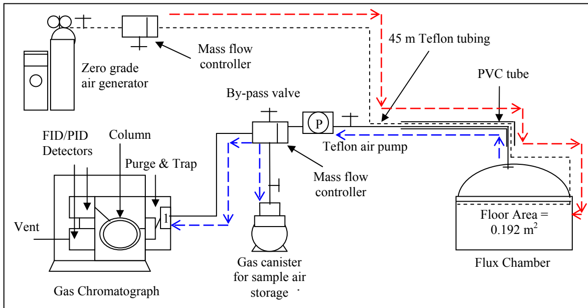
Figure 3. The schematic setup for VOC/ROG field measurements.
